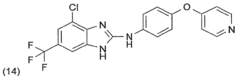
(4-Chlor-6-trifluormethyl-1H-benzimidazol-2-yl)-[4-(pyridin-4-yloxy)-phenyl]-amin
